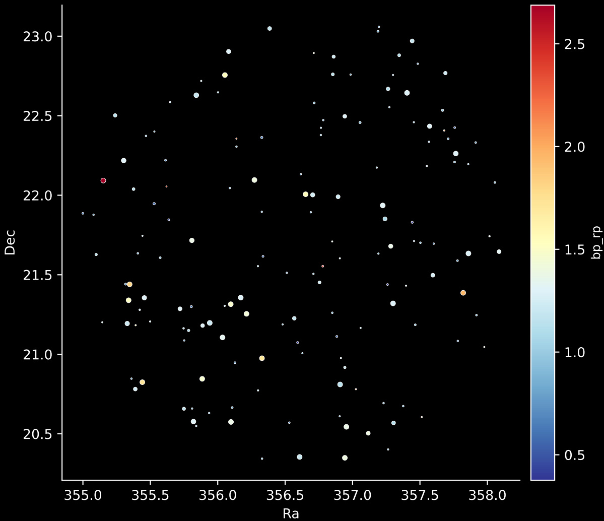
APOGEE DR17 Field: [043+32_MGA] Stars: 156
