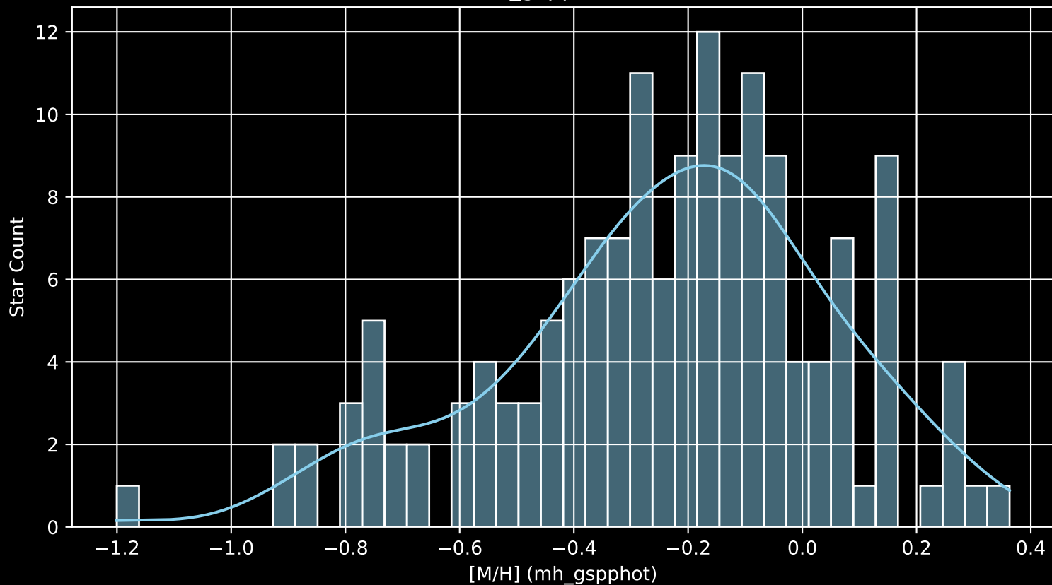
APOGEE DR17 Field: [043+32_MGA [M/H] (mh_gspphot) (n= 154)
