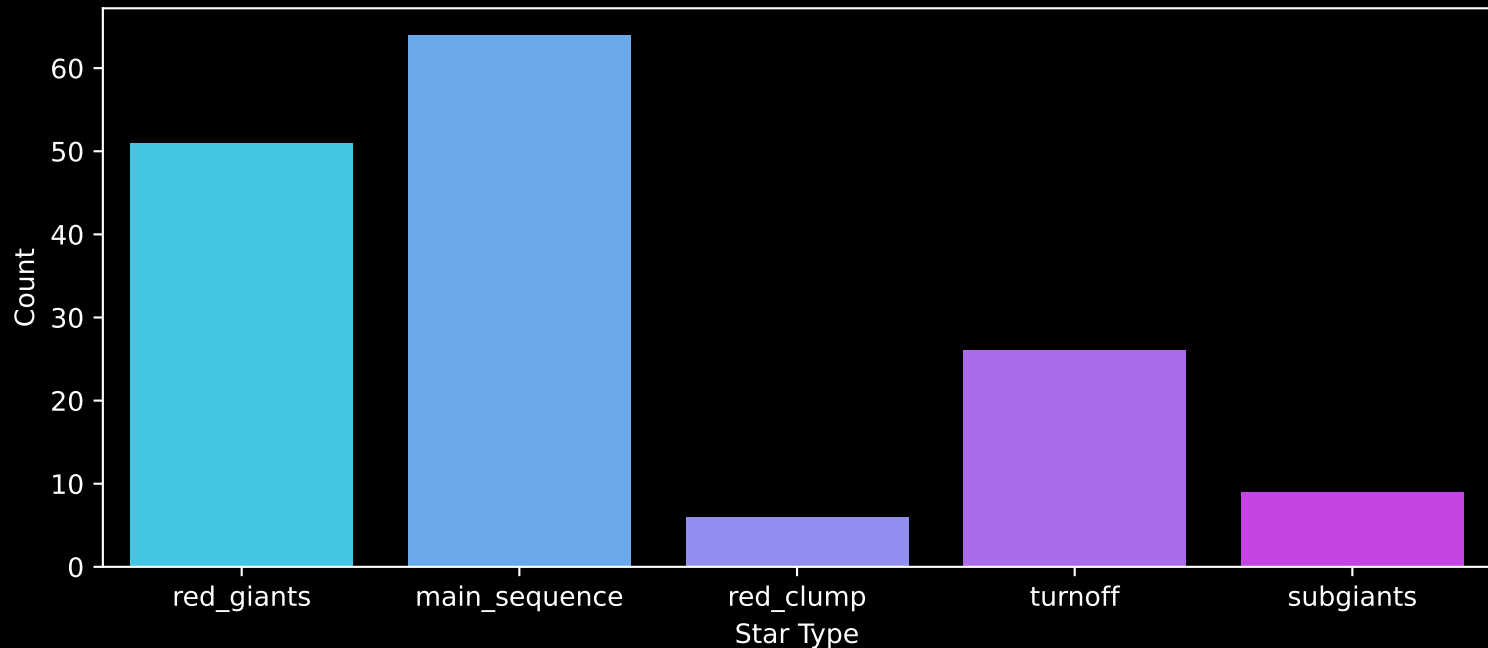
APOGEE DR17 Field: [043+32_MGA] Count plot of Star Type
