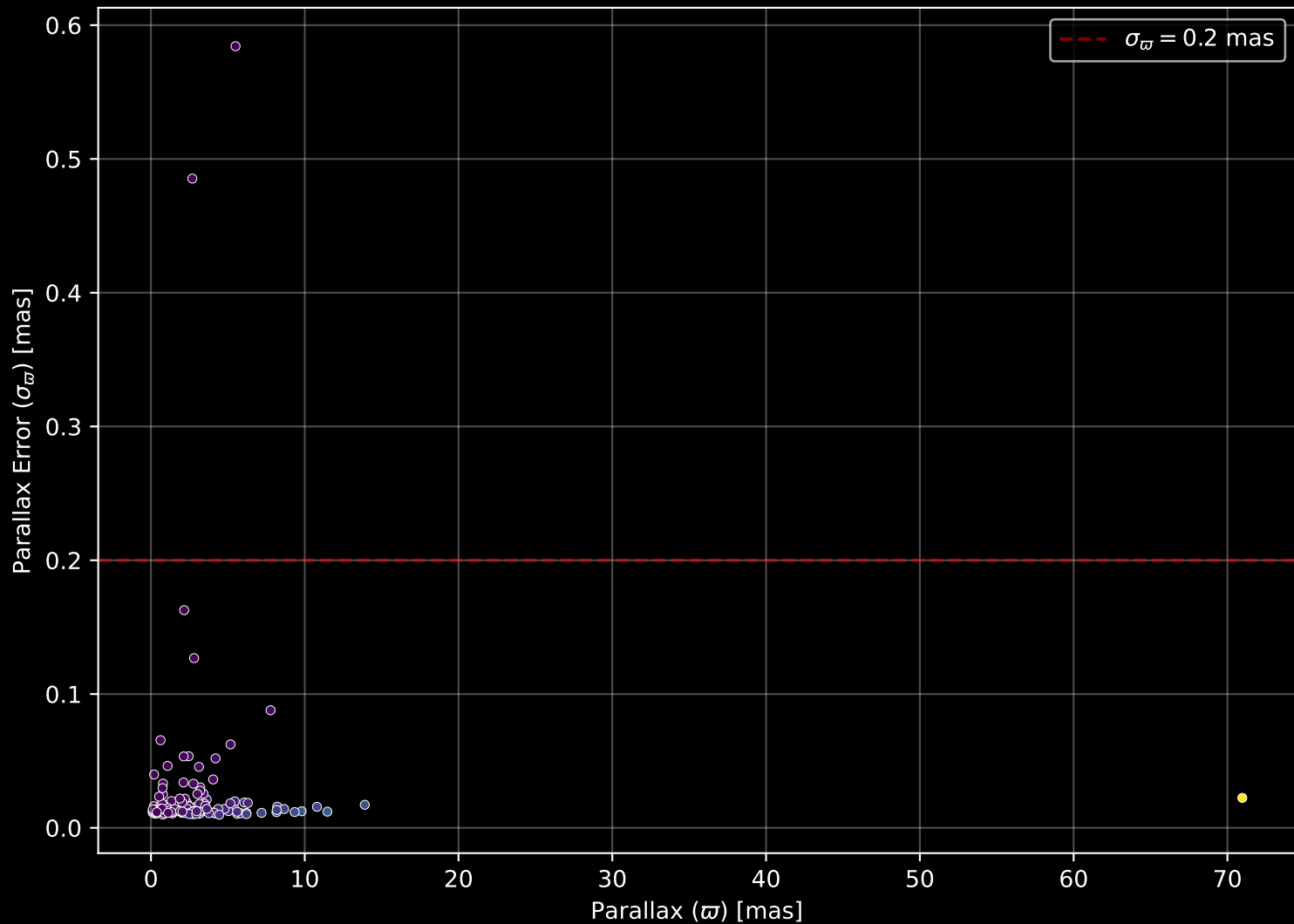
APOGEE DR17 Field: [043+32_MGA] Parallax Quality (n= 156)
