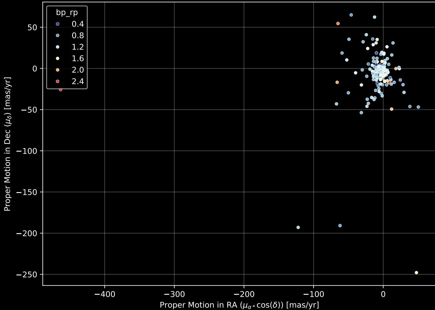
APOGEE DR17 Field: [043+32_MGA] Proper Motion Diagram (n= 156)
