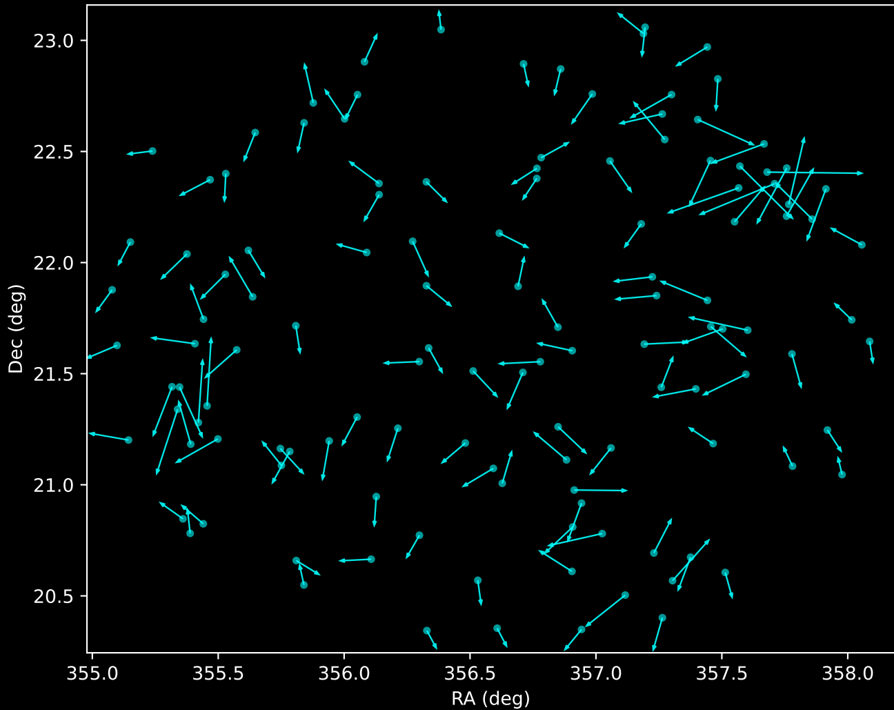
APOGEE DR17 Noise Stream Proper Motion Vectors (n=125)
