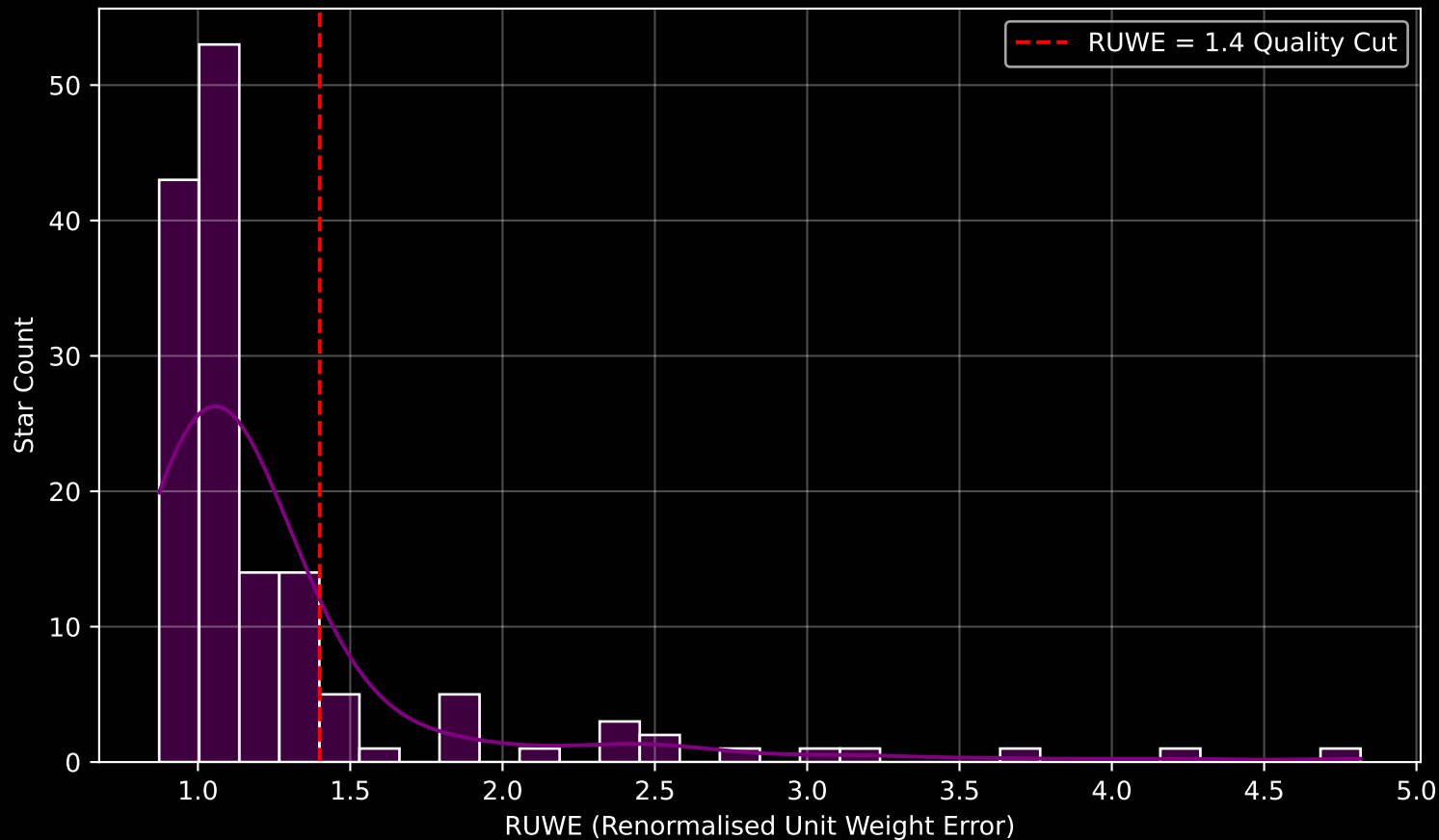
GAPOGEE DR17 Field [043+32_MGA] RUWE Distribution (n= 147)
